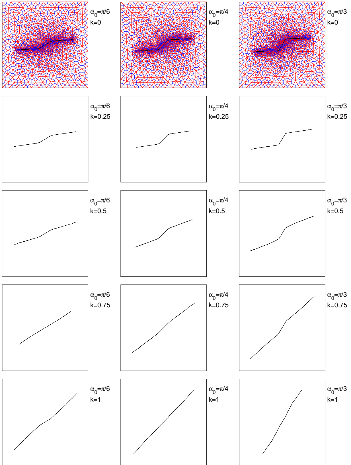
Figure 9: Crack trajectory for \mathbf{a}_0 = \mathbf{p}/6, \mathbf{p}/4, \mathbf{p}/3 , and k = 0, 1/4, 1/2, 3/4, 1 .
