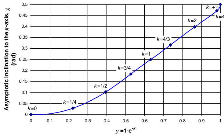
Figure 11: Relation between the angle g and the variable y .
