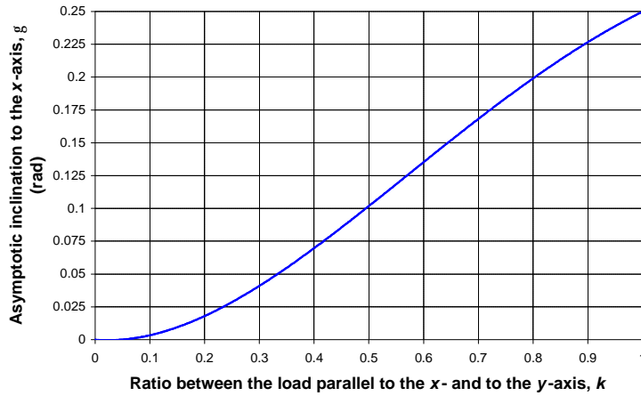
Figure 10: Relation between the angle g and the ratio k .
