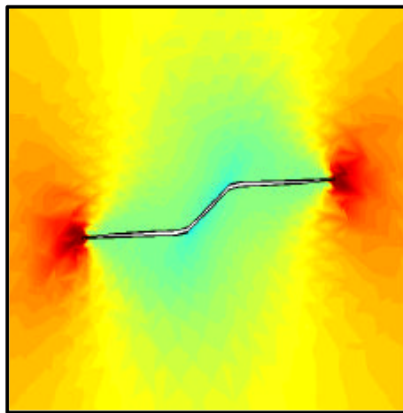
Figure 7: 2D p_y analysis for a generic propagation step with k=0 , \mathbf{a}_0 = \mathbf{p}/4 .
